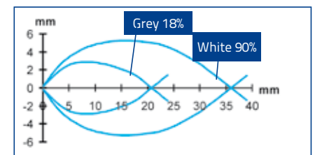
Detection area - proximity *
