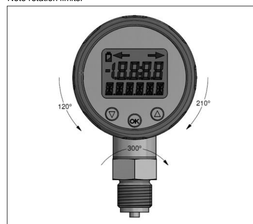
Fig. 2 Rotatability
