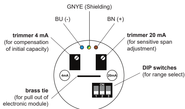
The top view on the internal electronic module with current output (variant -I)
