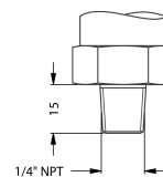
1/4" NPT
